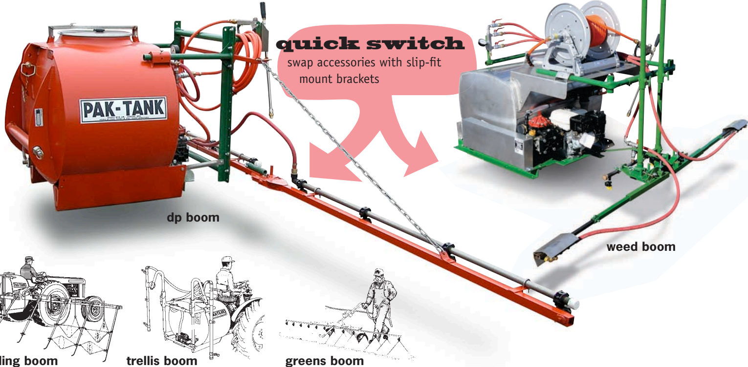
trailing boom
